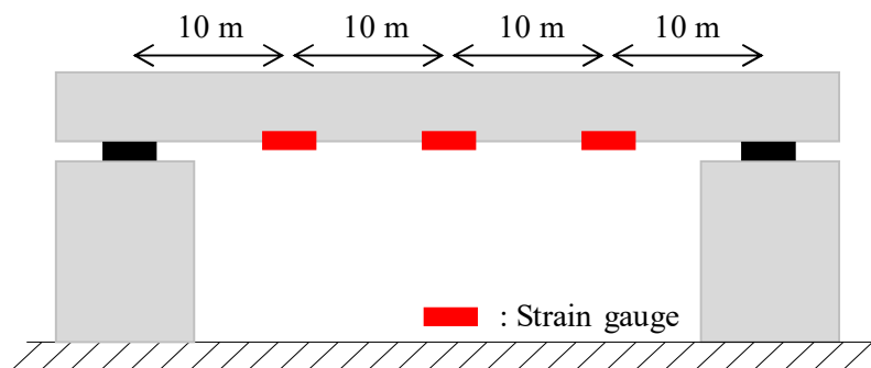
(b) Deployment scheme of the strain gauges
