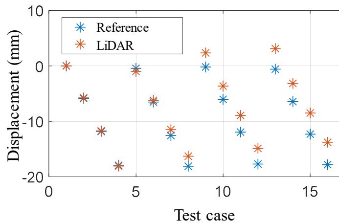
(b) Test results with different LiDAR position
