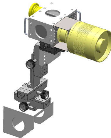
Figure 61. An example of three-dimensional model for dual-camera system.
