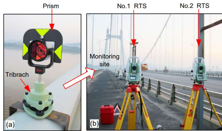
(a) Displacement measurement using a robotic total station [111]
