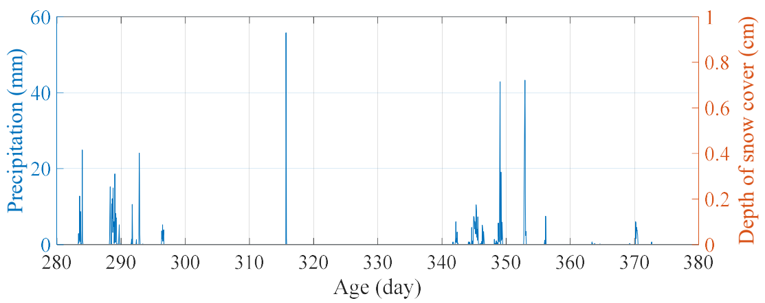
(c) Precipitation and depth of snow cover (Age of 280–380 days)
