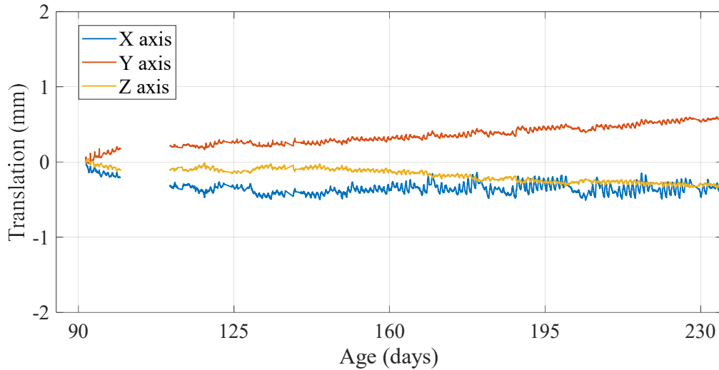
(a) Translational camera motion
